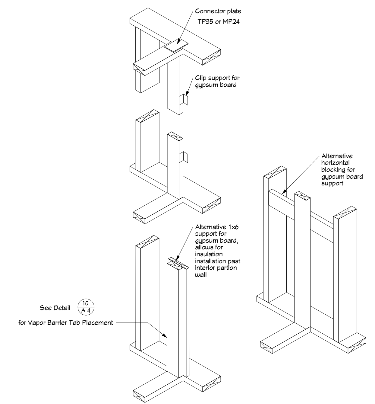
4 FRAMING DETAIL OPTIONS
