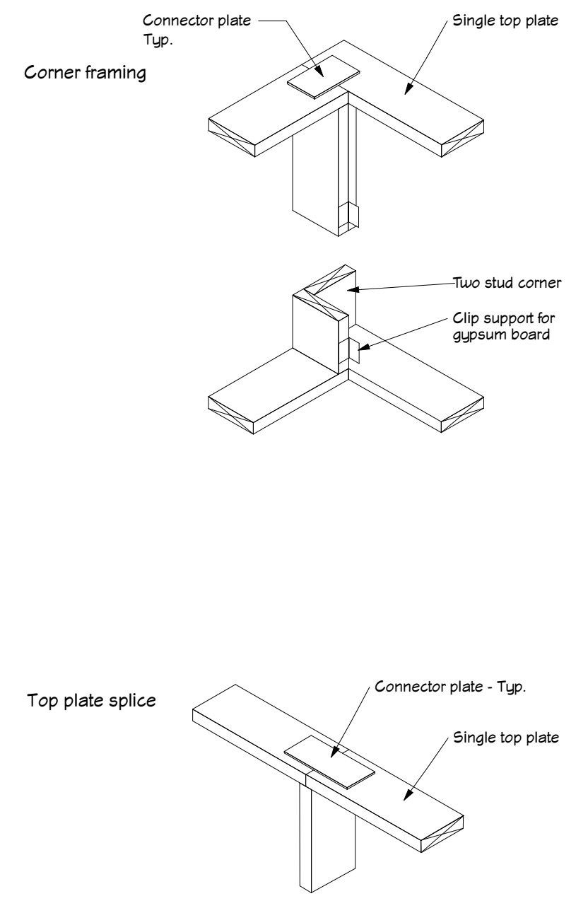
3 SPLICE DETAILS
