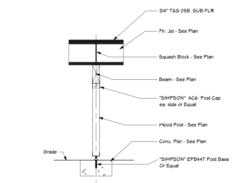
7 POST & PIER DETAIL
