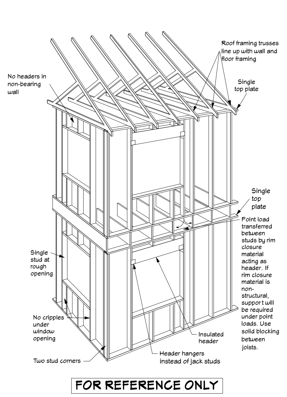
1 FRAME OVERVIEW
