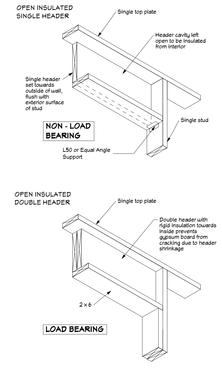
5 HEADER DETAIL OPTIONS
